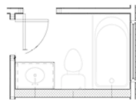
ENLARGED BATH 2 PLAN
