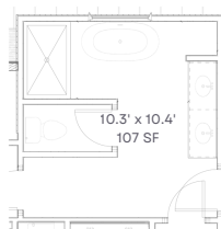
ENLARGED BATH 2 SCALE 1/4" = 1'-0"
