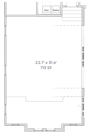
LVL 1 - CART GARAGE OPT SCALE 1/4" = 1'-0"
