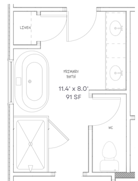
ENLARGED PRIMARY BATH SCALE: 1/2" = 1'-0"
