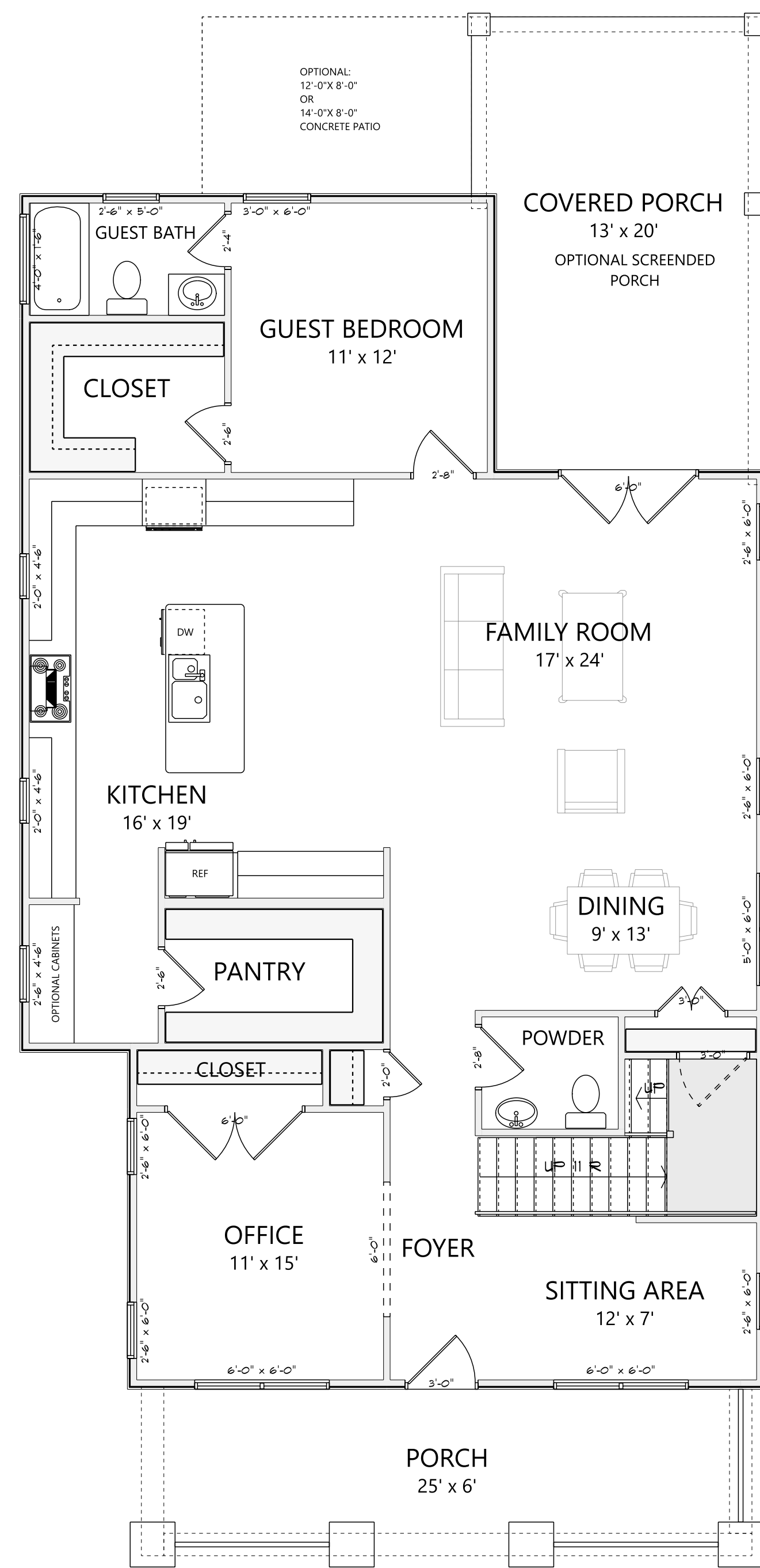
MAIN LEVEL ELEVATION A 1551 HEATED SQ FT
