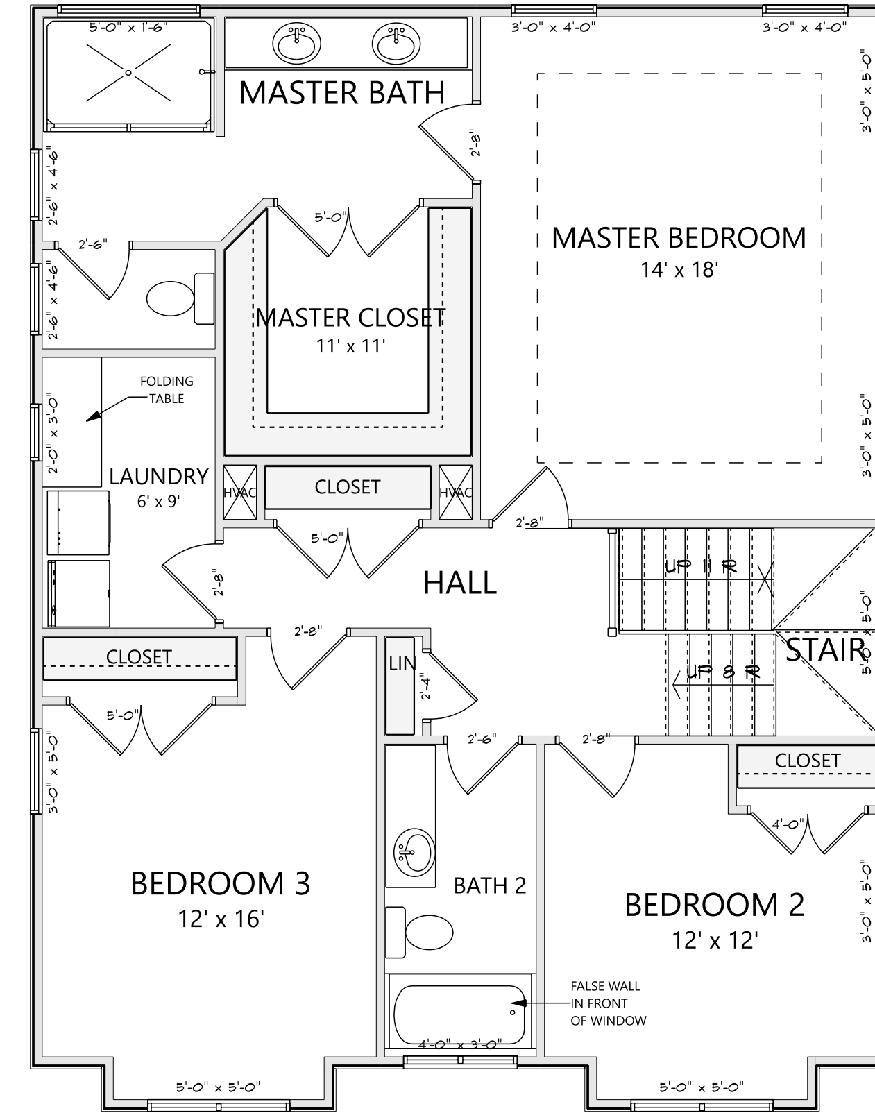
UPPER LEVEL ELEVATION A 1139 HEATED SQ FT
