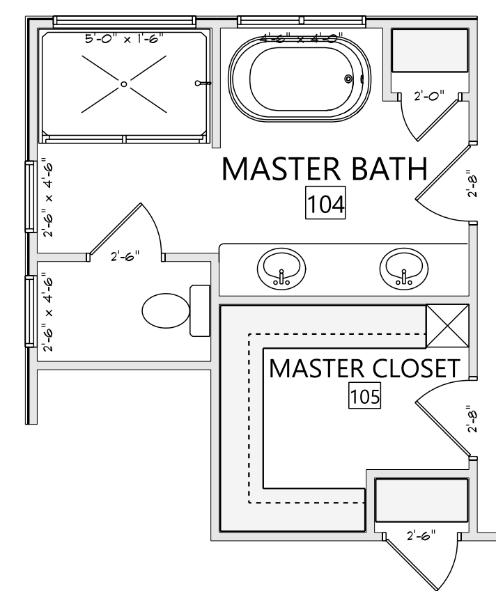
MASTER BATH OPTION 2
