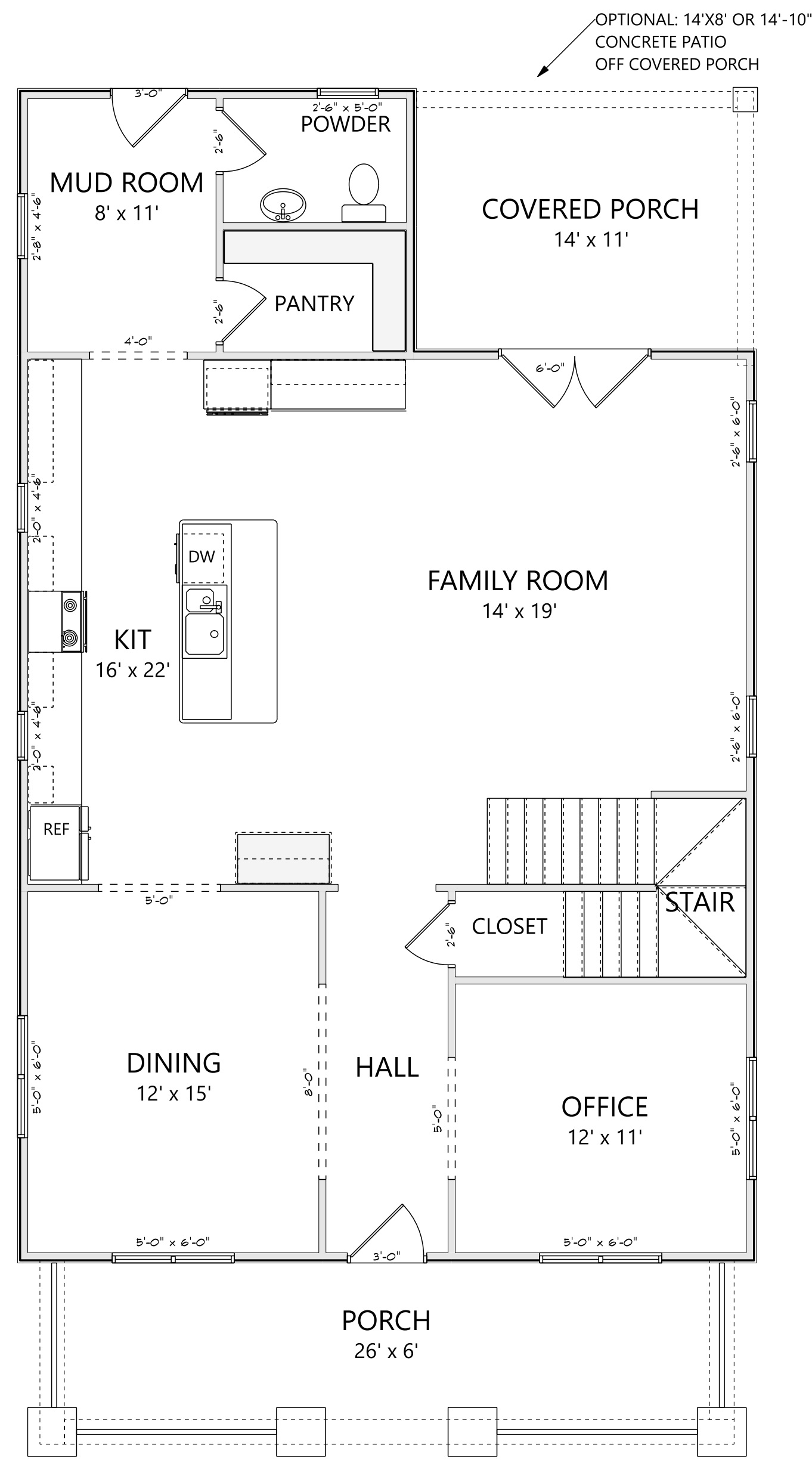
MAIN LEVEL ELEVATION A 1287 HEATED SQ FT
