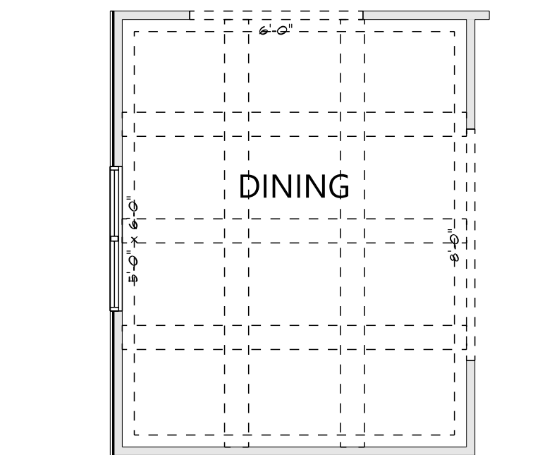
DINING COFFERED CEILING OPTION
