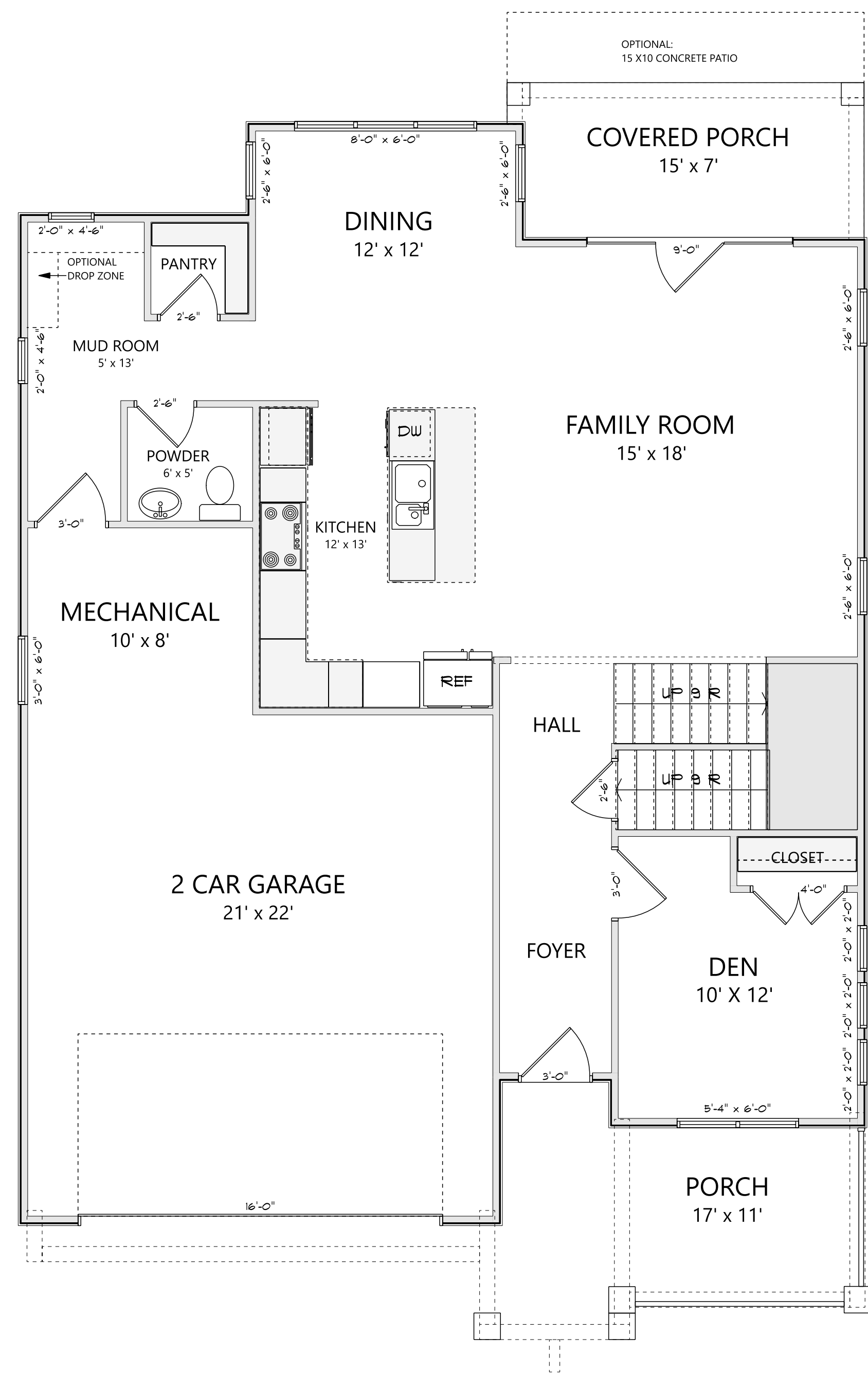
MAIN LEVEL ELEVATION A 1056 HEATED SQ FT
