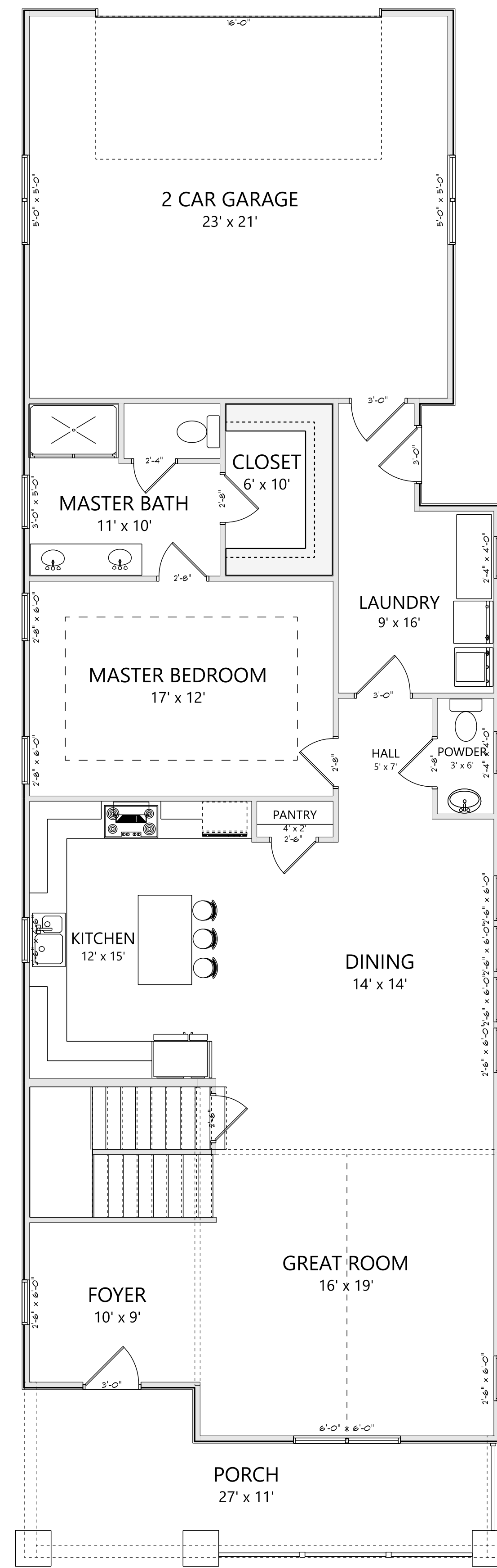
MAIN LEVEL ELEVATION A 1505 HEATED SQ FT
