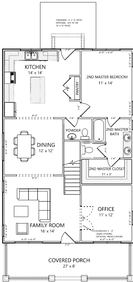
MAIN LEVEL ELEVATION A 1179 HEATED SQ FT
