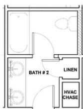
ENLARGED PLAN BATH OPT 2
