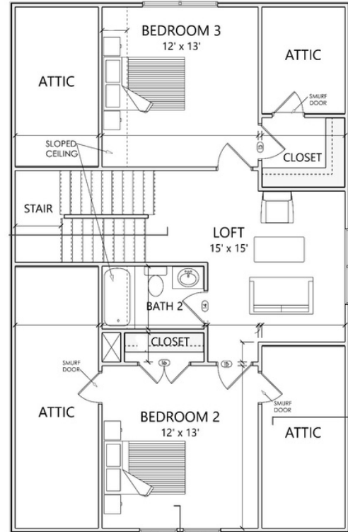
UPPER LEVEL
