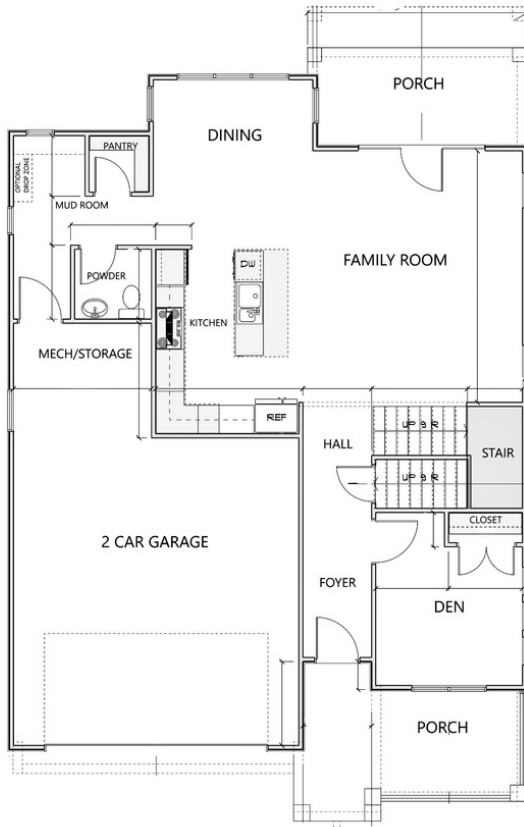
MAIN LEVEL
