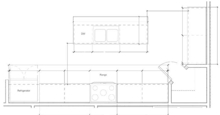
ENLARGED KITCHEN PLAN
