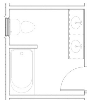
ENLARGED BATH 2 PLAN
