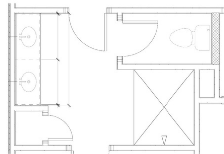
ENLARGED PRIMARY BATH PLAN
