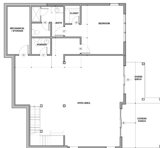
1 BASEMENT PLAN SCALE: 1/4" = 1'-0"
