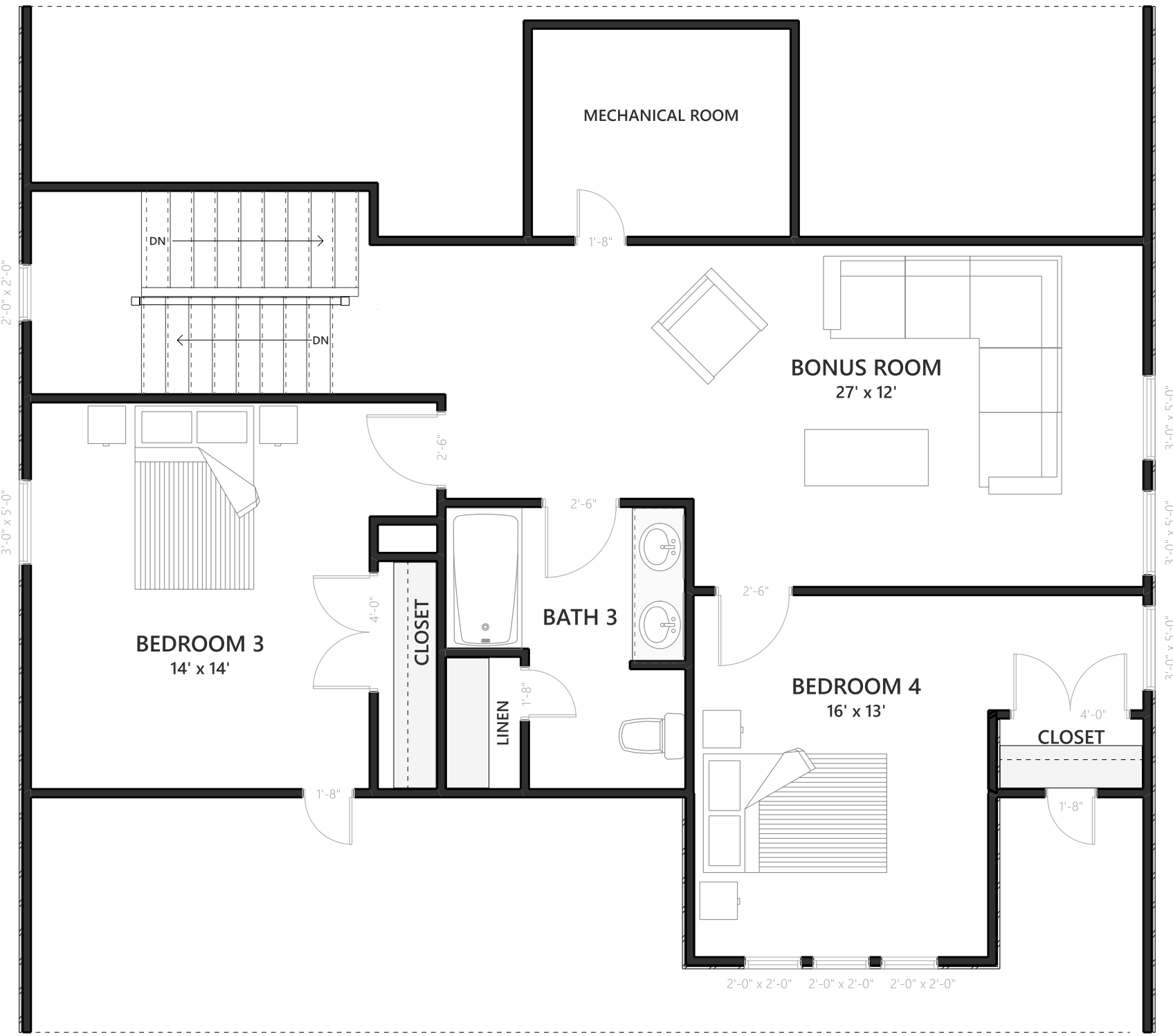
UPPER LEVEL ELEVATION A 804 HEATED SQ FT
