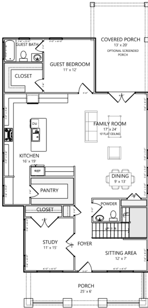
MAIN LEVEL ELEVATION A 1551 HEATED SQ FT
