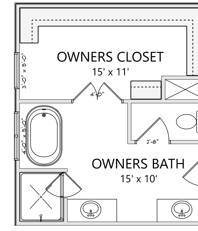
OWNERS BATH OPTION 2
