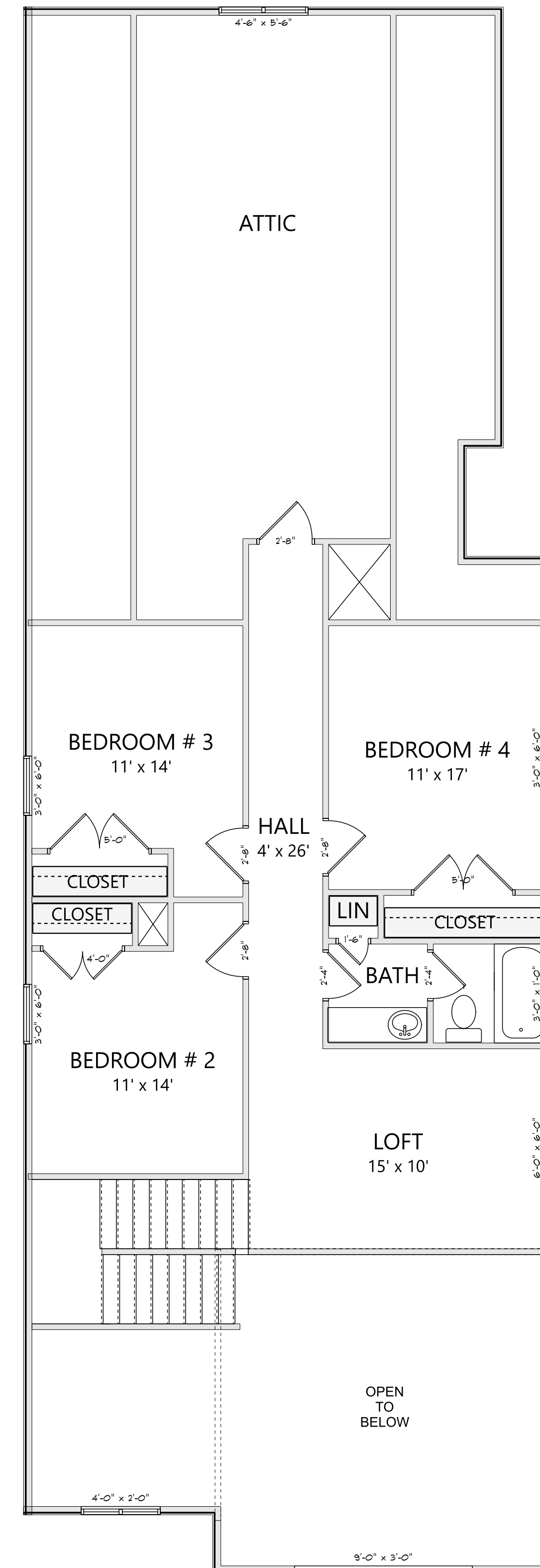
UPPER LEVEL ELEVATION B 1245 HEATED SQ FT
