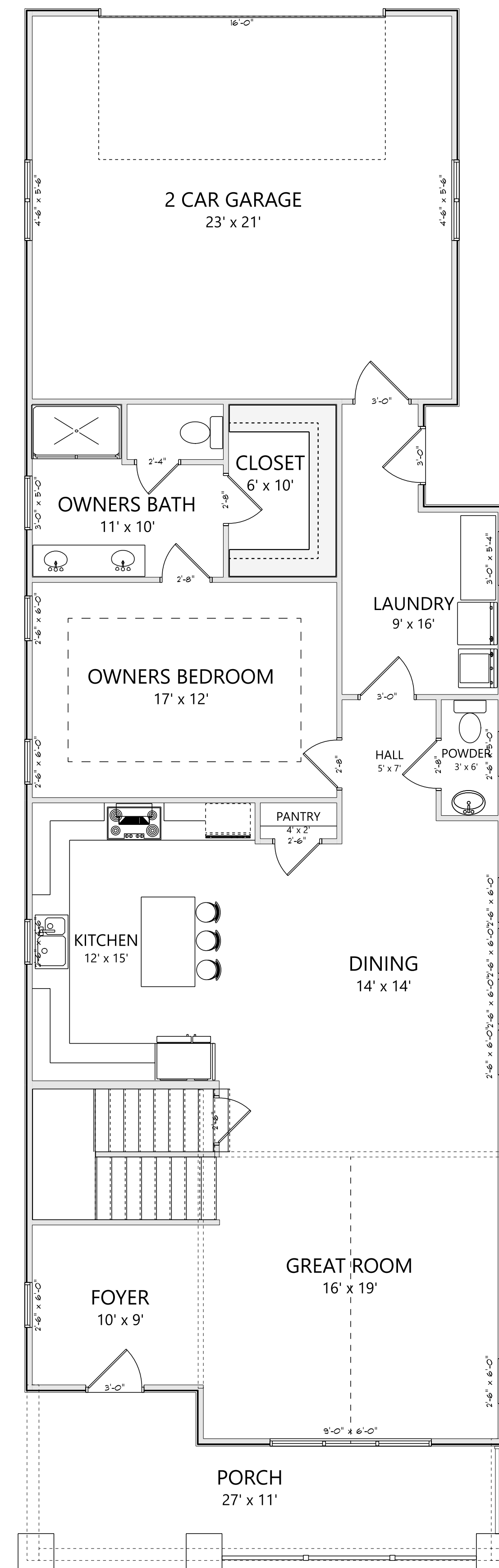
MAIN LEVEL ELEVATION B 1505 HEATED SQ FT
