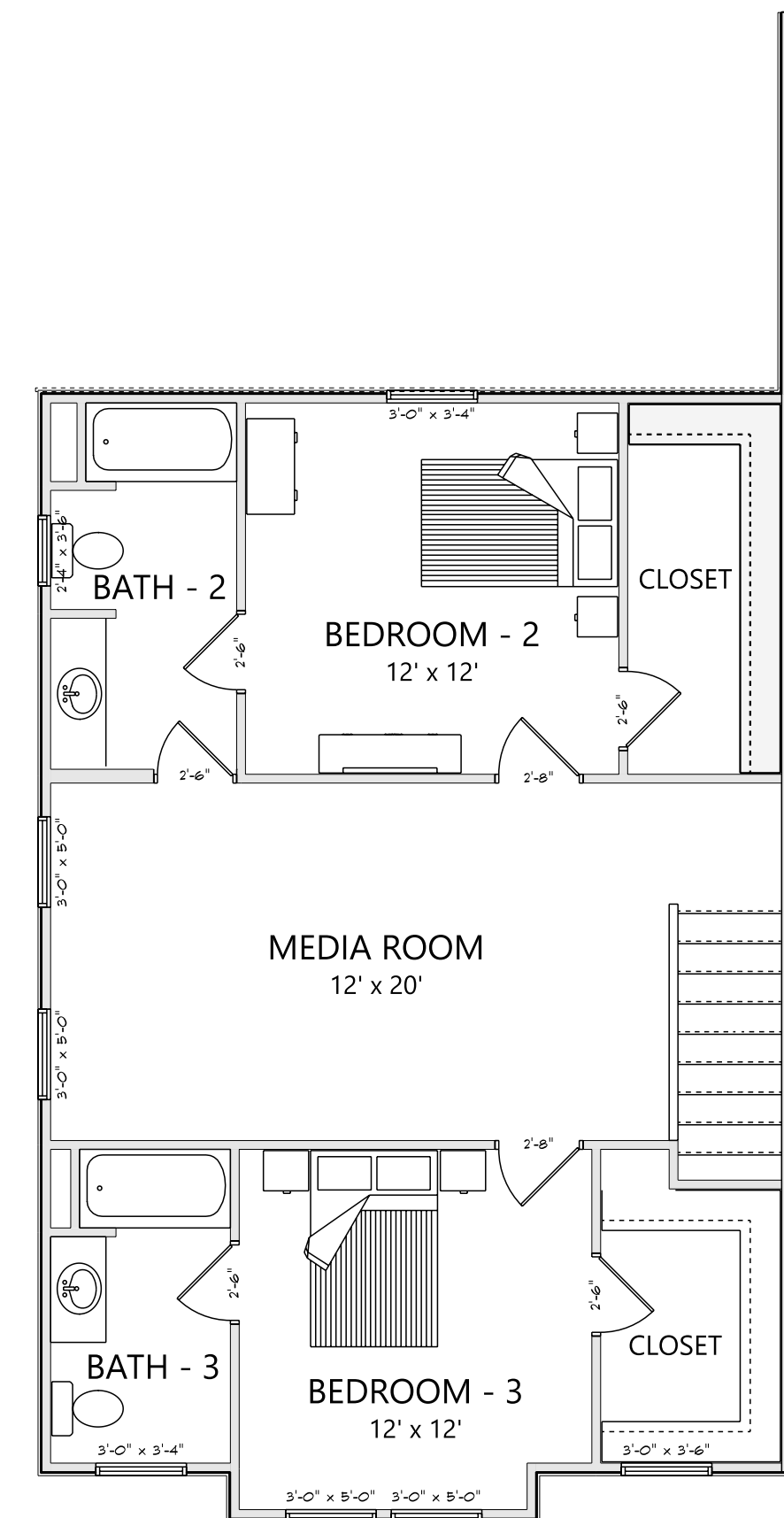
SECOND FLOOR 908 HEATED SQ FT
