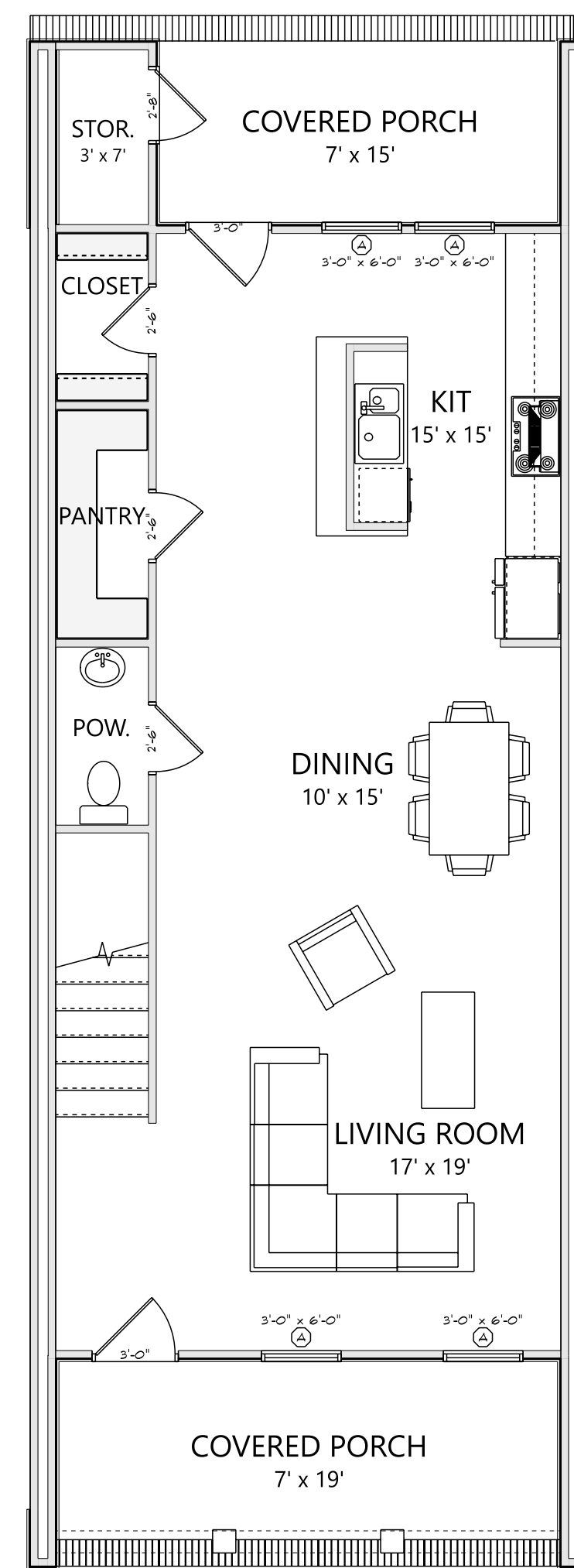
FIRST FLOOR 855 HEATED SQ FT
