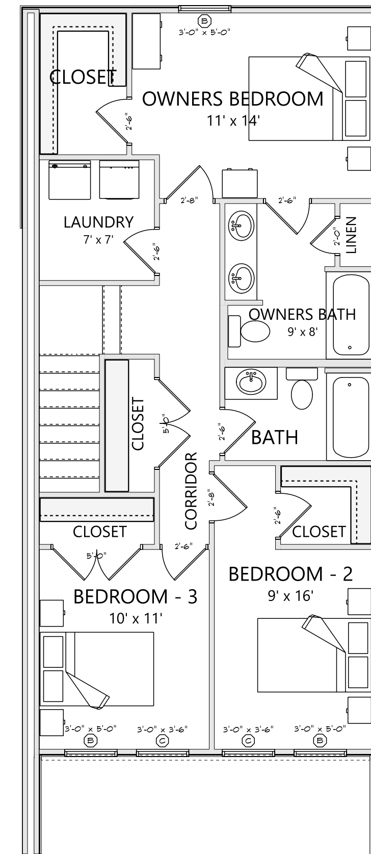
SECOND FLOOR 852 HEATED SQ FT
