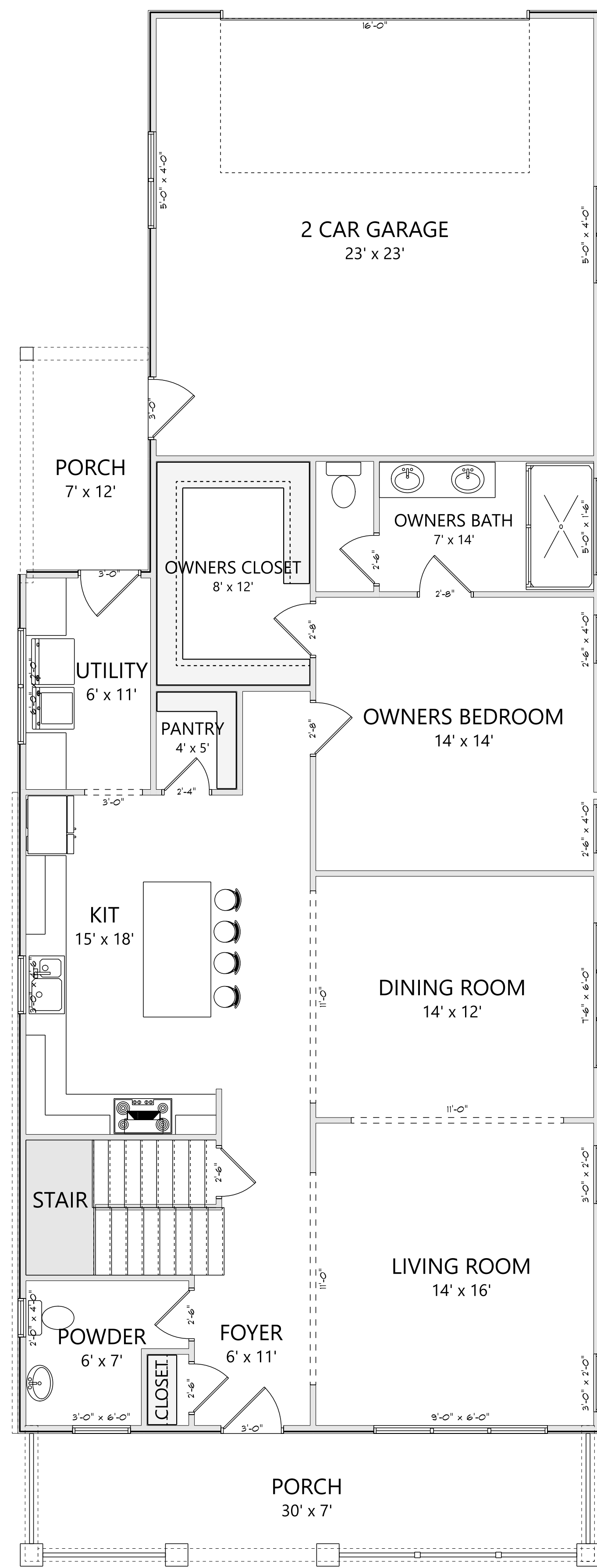
MAIN LEVEL 1493 HEATED SQ FT TOTAL DIMENSIONS - 30'-0" X 80'-6"
