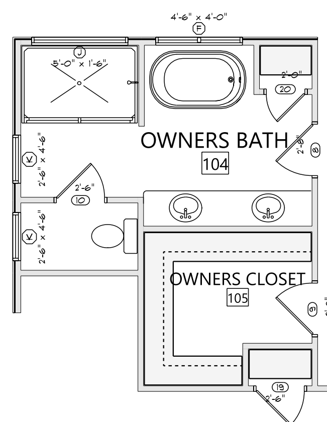
OWNERS BATH OPTION 2
