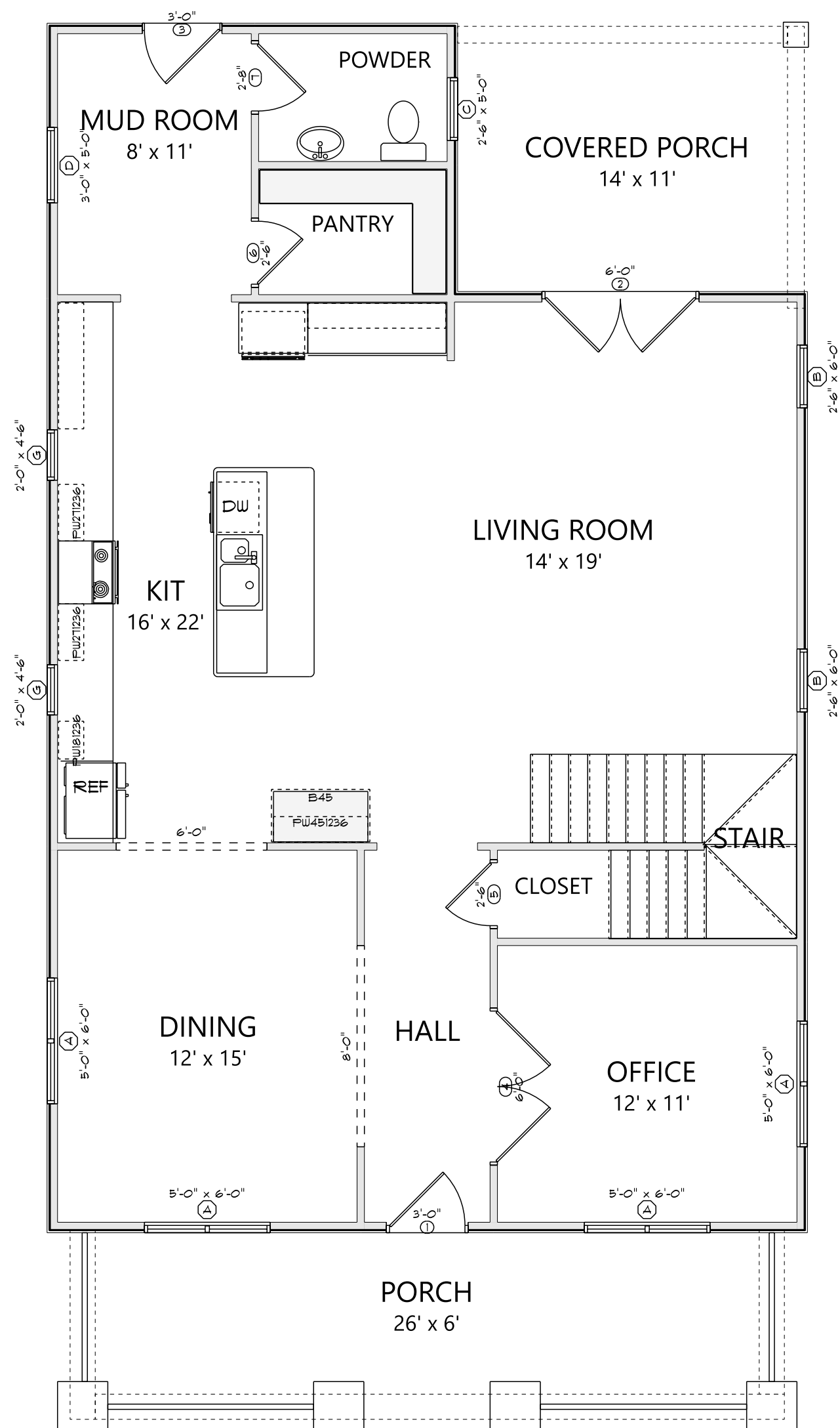
MAIN LEVEL ELEVATION A 1287 HEATED SQ FT TOTAL DIMENSIONS - 30'-0" X 56'-0"
