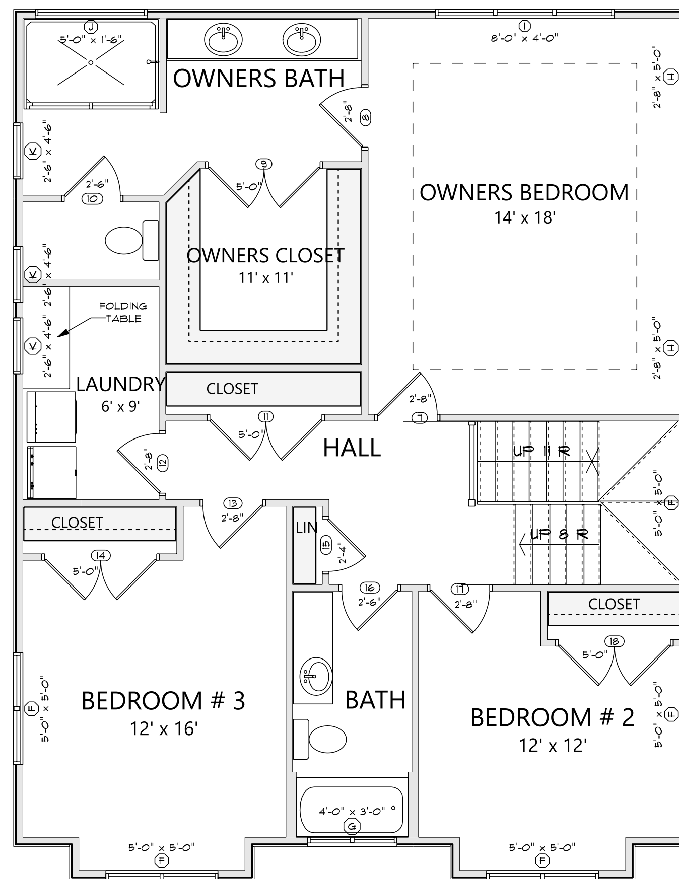
UPPER LEVEL ELEVATION A 1139 HEATED SQ FT
