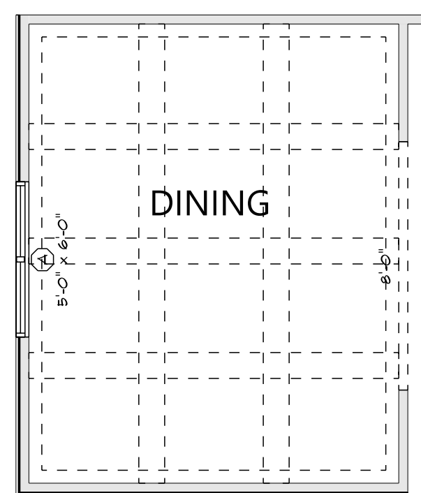
DINING COFFERED CEILING OPTION
