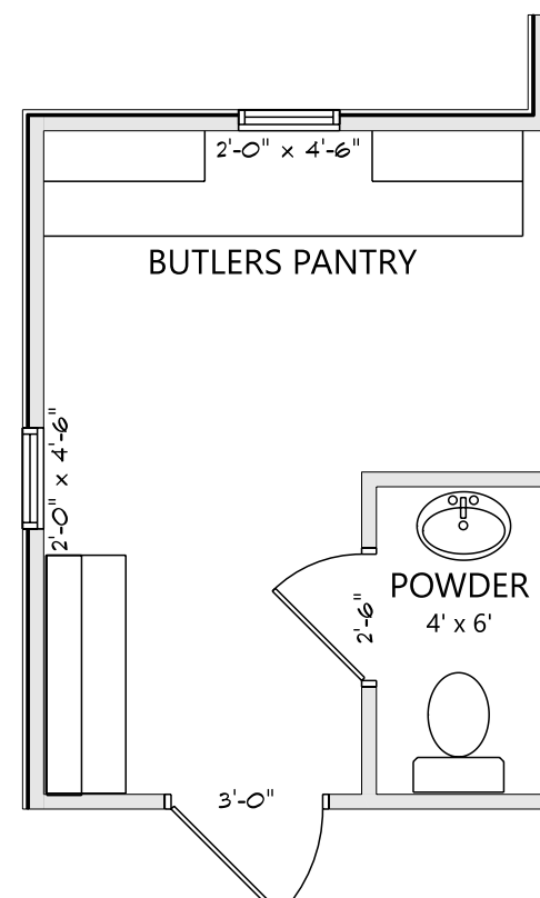
BUTLERS PANTRY OPTION 1
