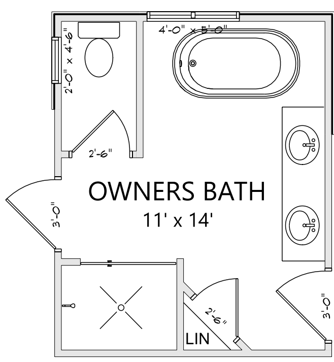
OWNERS BATH OPTION 2
