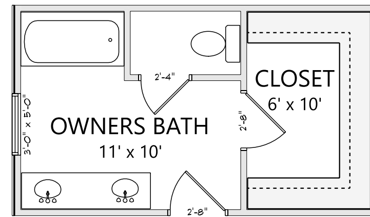
OWNERS BATH OPTION 2
