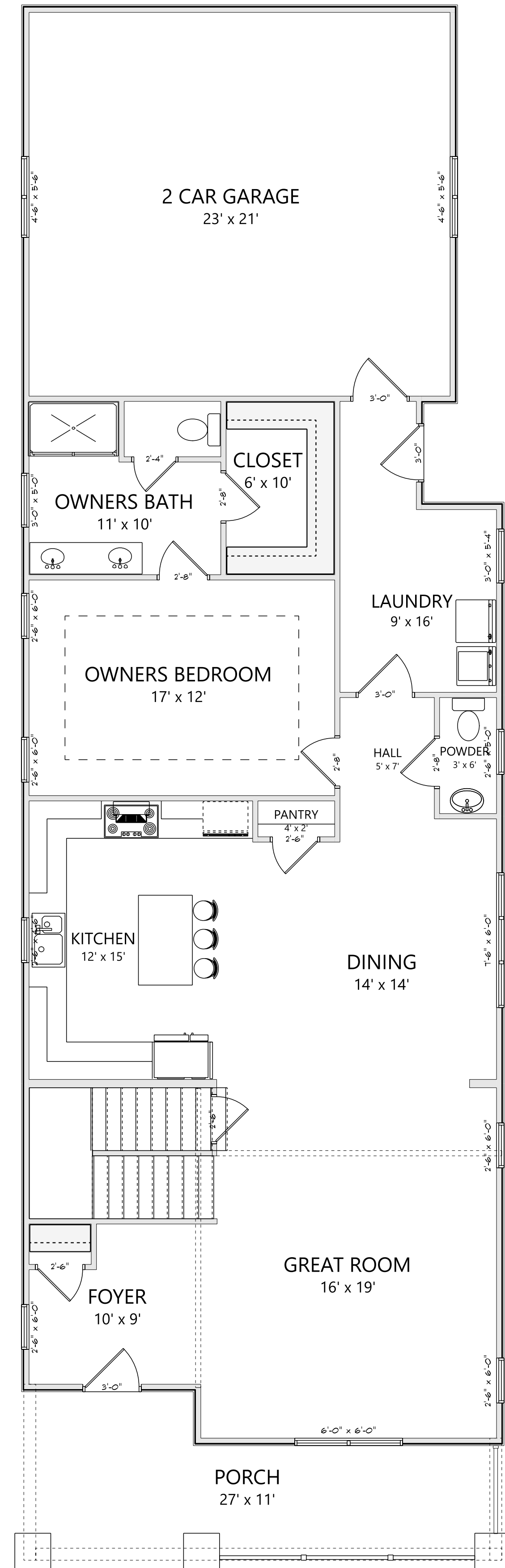
MAIN LEVEL ELEVATION B 1503 HEATED SQ FT
