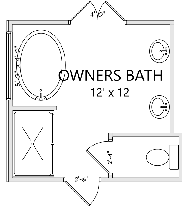
OWNERS BATH OPTION 2
