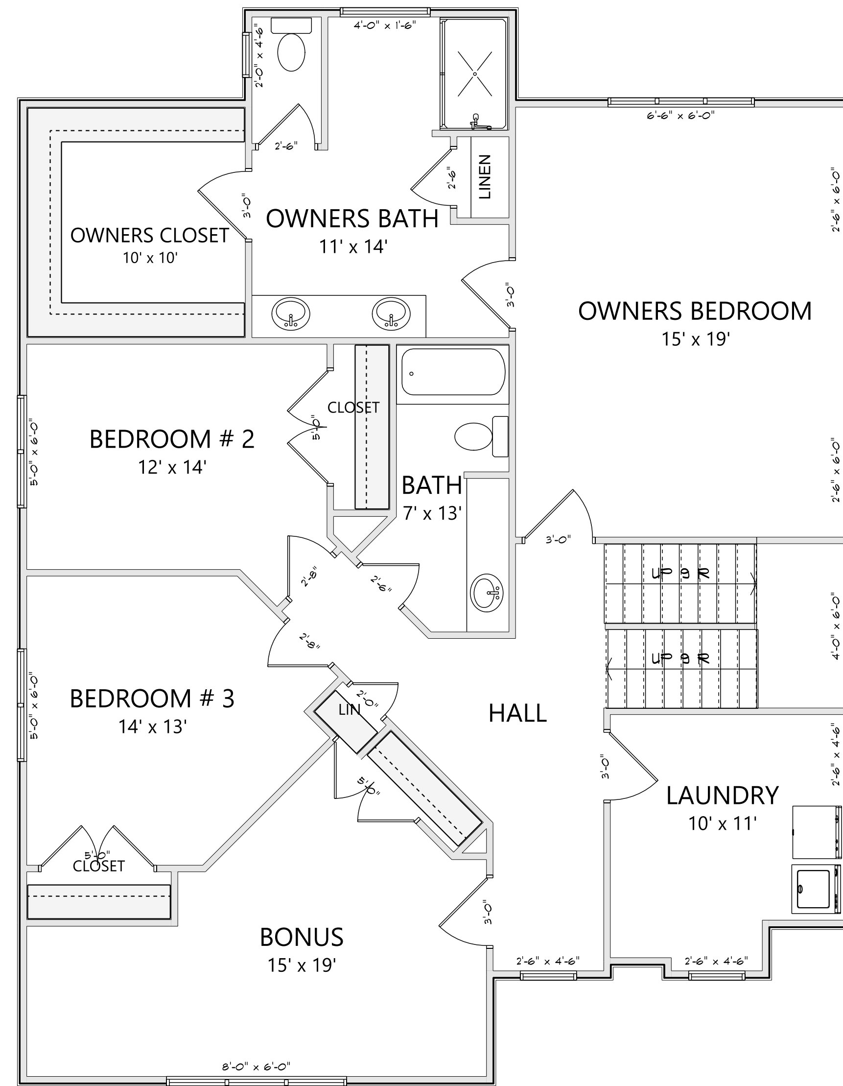
UPPER LEVEL ELEVATION B 1557 HEATED SQ FT
